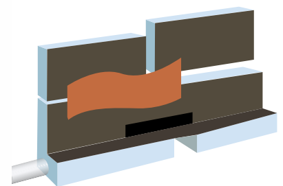
Waterproofing connection with integrated flange.
