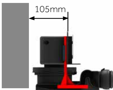
Minimal installation only 105 mm from base to finished tile floor.
